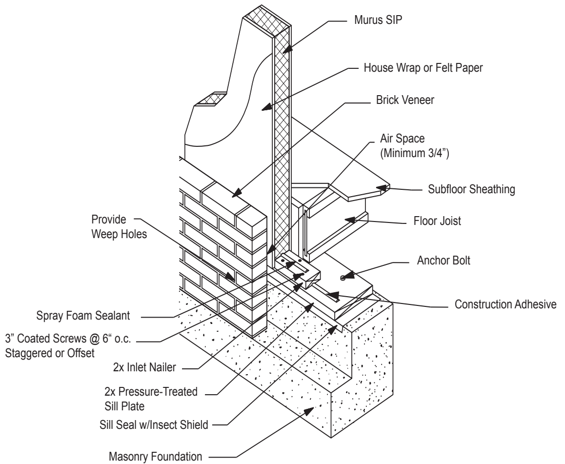
Figure 29. Veneer Detail
