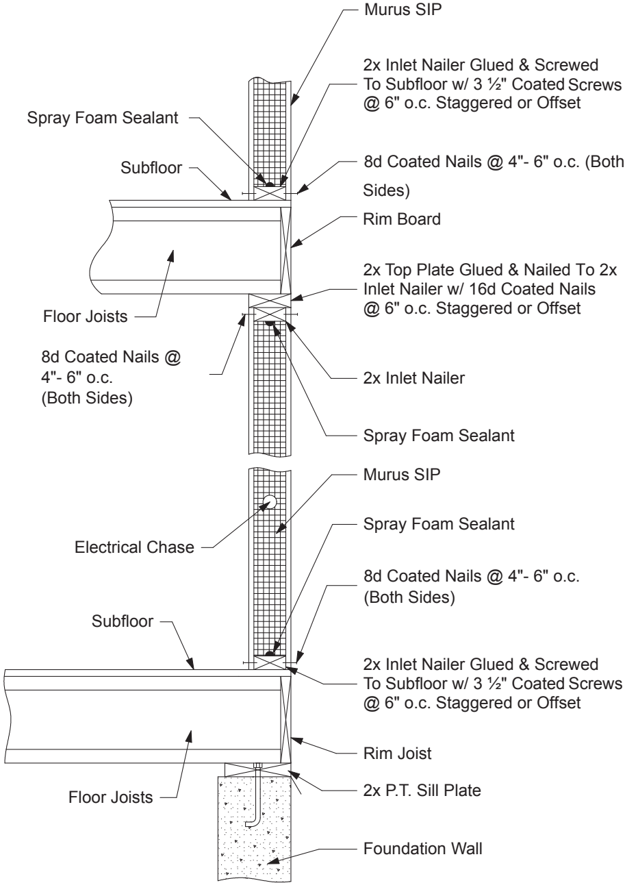
Figure 5B. Typical Wall Section with Platform Framed Floor Systems
