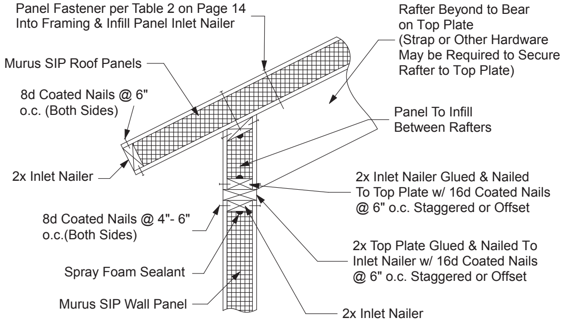
Figure 15. Typical rafter system detail
