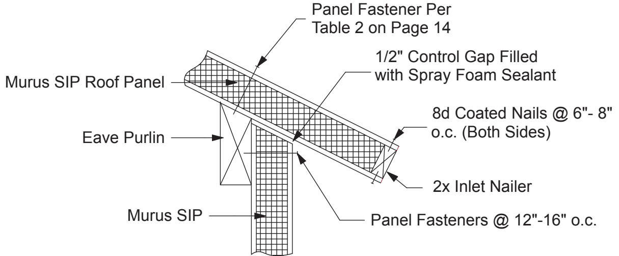
Figure 13E. Typical Eave Detail with Starter Purlin Roof System
