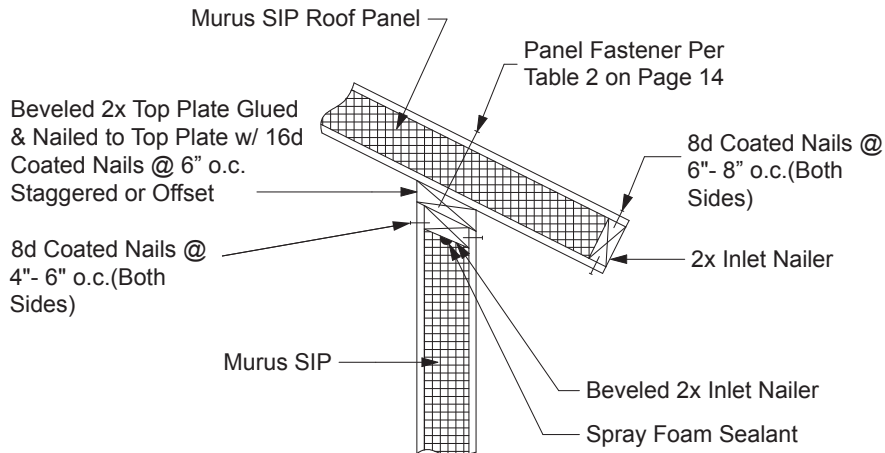
Figure 13D. Typical Eave Detail for Purlin System with Beveled Plate and Nailer
