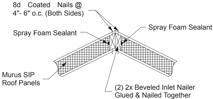
Figure 19C. Structural Ridge Details
