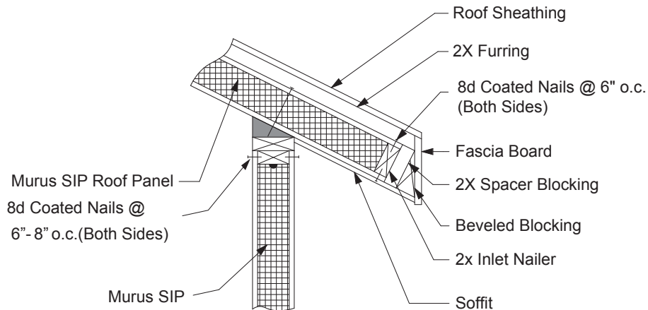
Figure 17B. Soffit and Fascia Options
