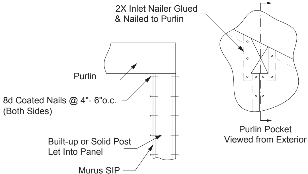
Figure 14A. Purlin Bearing Housing
