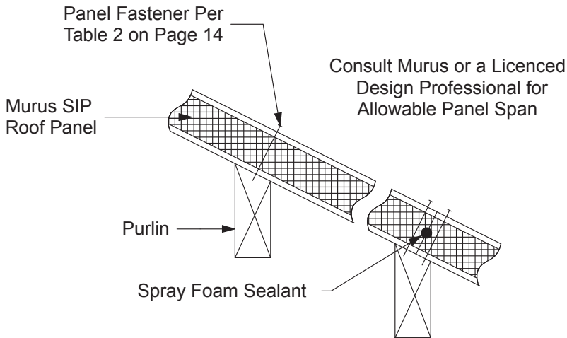
Figure 14B. Purlin Bearing Housing with Exposed Post
