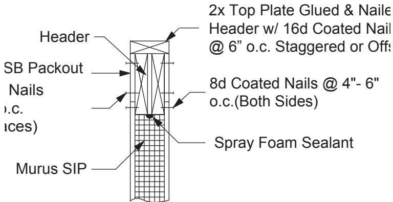
Figure 7C. Load Bearing Top Plate Header Connection Detail
