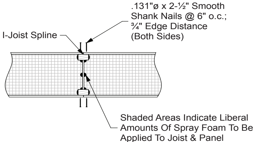
Figure 10F I-Joist Spline Used for joining roof panels where structural reinforcement is required
