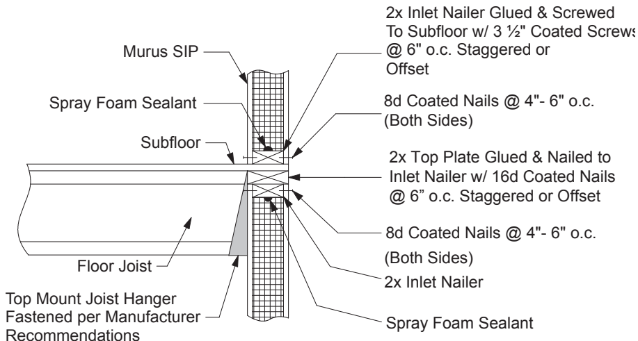
Figure 8A. Hung Joist Floor System
