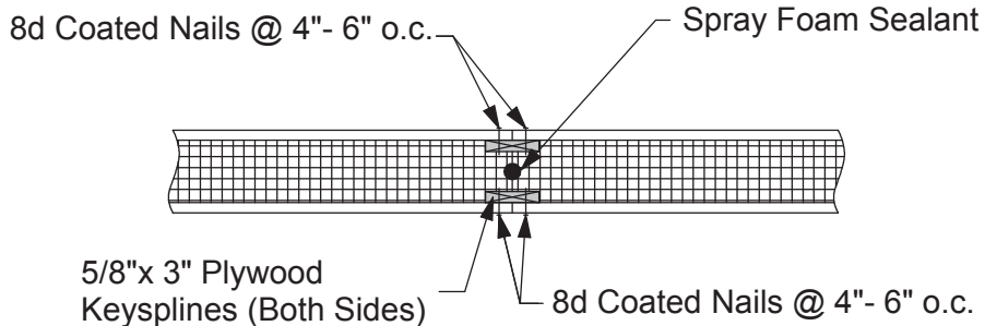
Figure 6C. Double Key Spline Connection Detail
