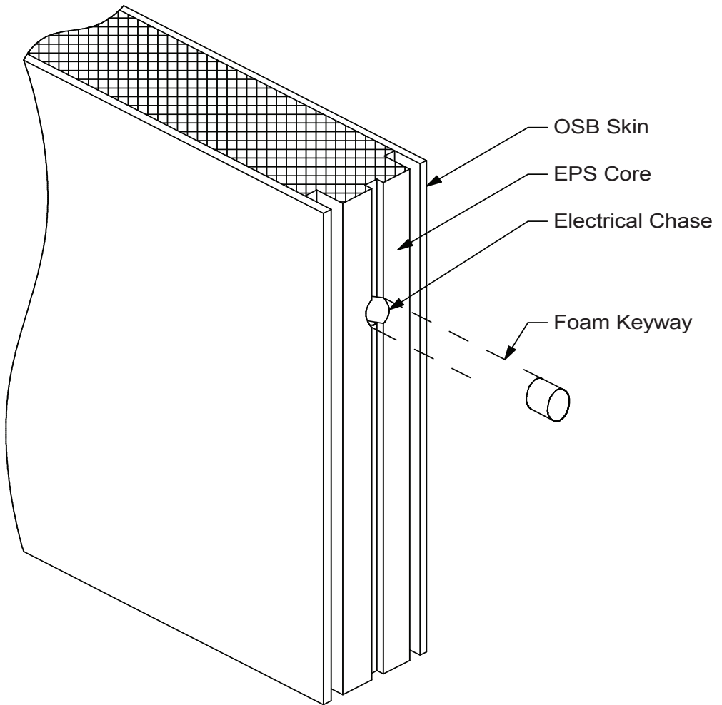
Figure 6D. Chase Tube Insert Application
